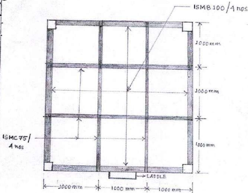
PLAN OF PLATFORM
