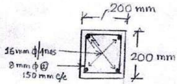
Fig: Column (C 1 ) (200 x 200) mm
