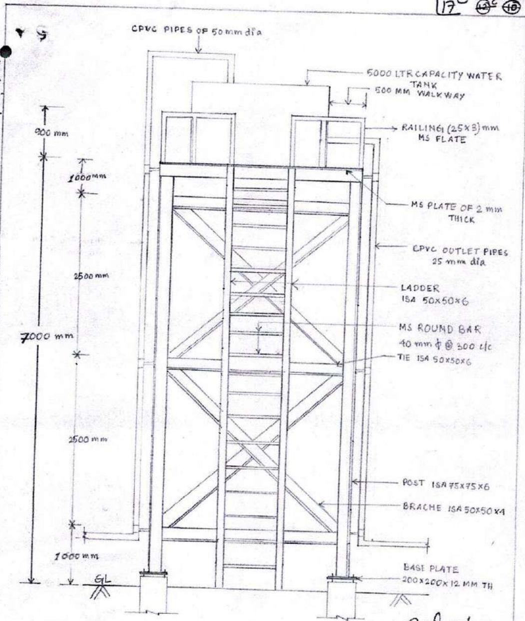
ELEVATION OF WATER STAGING
