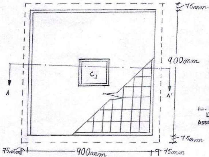
PLAN OF FOOTING
