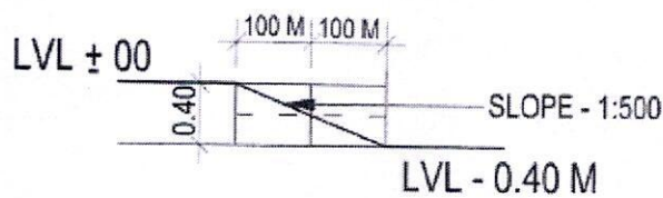
LONGITUDINAL SECTION OF DRAIN 2
