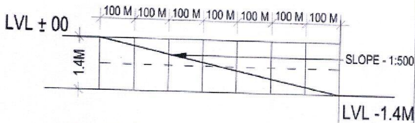
LONGITUDINAL SECTION OF DRAIN 1
