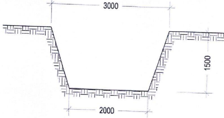
CROSS SECTION OF DRAIN 1
