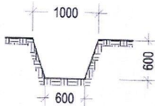
CROSS SECTION OF DRAIN 2
